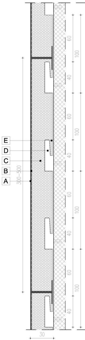
SECTION B-B
